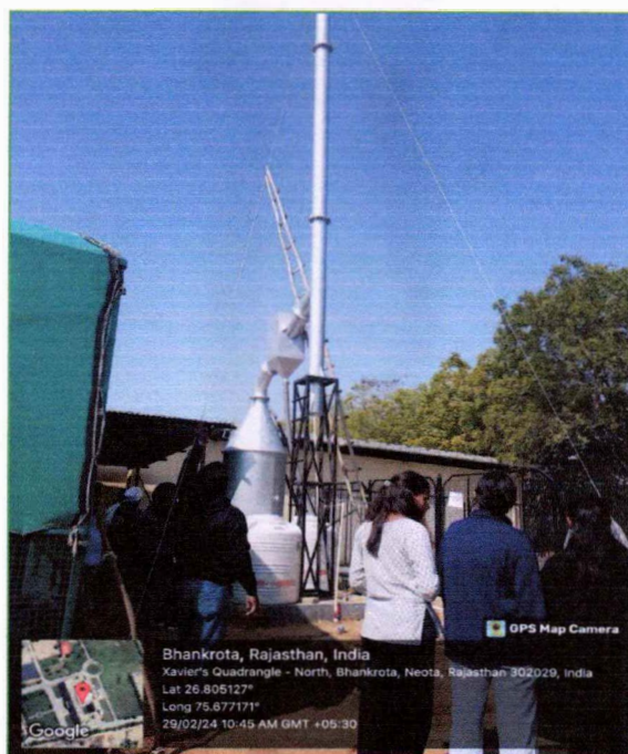
Incinerator
