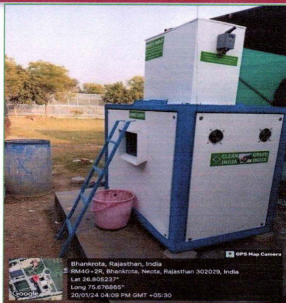
Bio-Compost Machine
